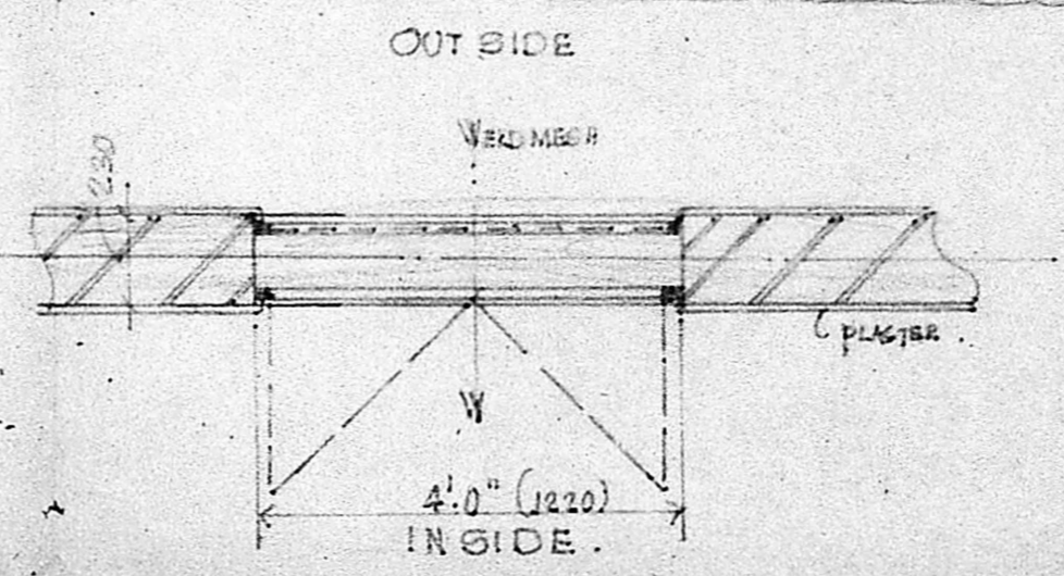
TYP. DETAIL OF WINDOW & WELDMESH ARRANGEMENTS.
