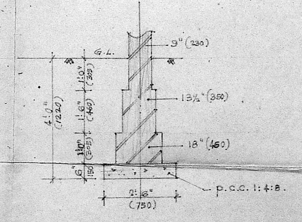
TYP. FDN. DETAIL OF 230TK BRICK WALL (3")
