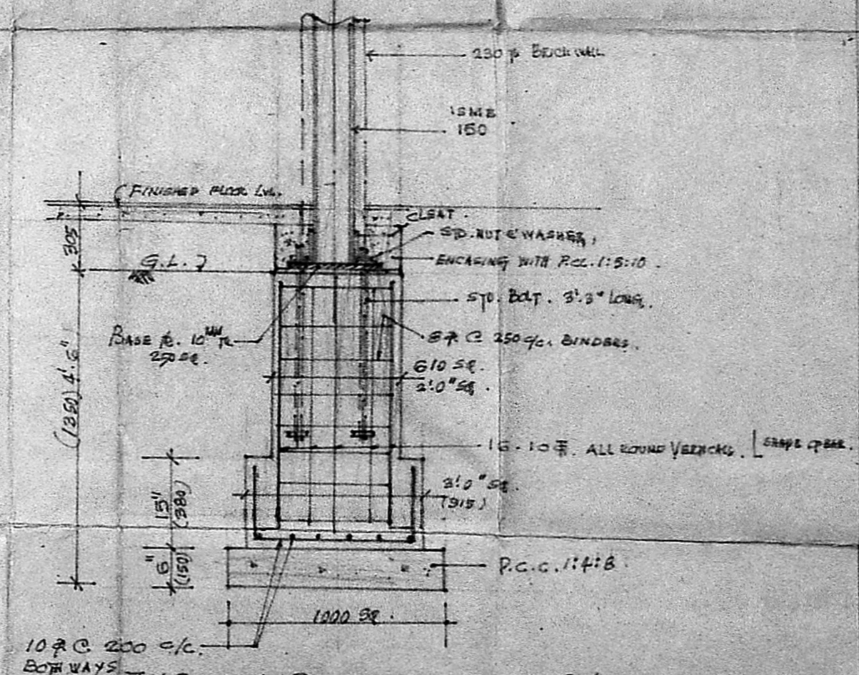
TYP. FDN. DETAILS OF STEEL COL. (15MB 150)
